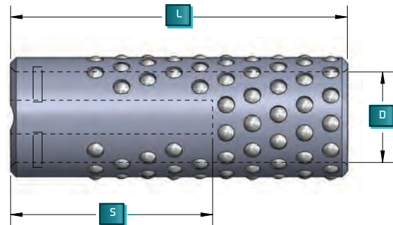
BALL BEARING CAGES - DIAMETER 50-80
