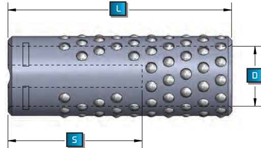
BALL BEARING CAGES - DIAMETER 1 3/4" - 3"
